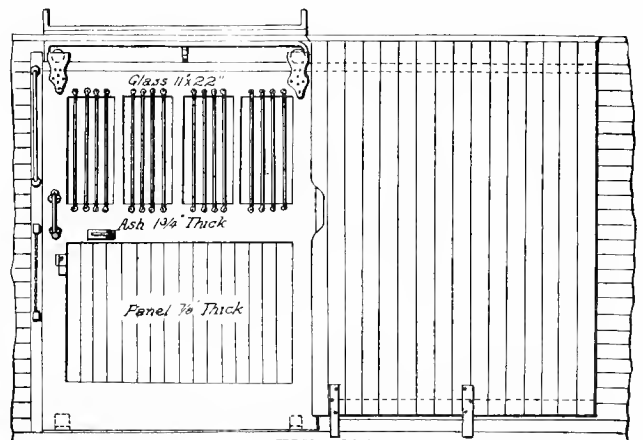
Fig. 1793. BAGGAGE-CAR SIDE-DOOR. NEW YORK CENTRAL & HUDSON RIVER RAILROAD.
